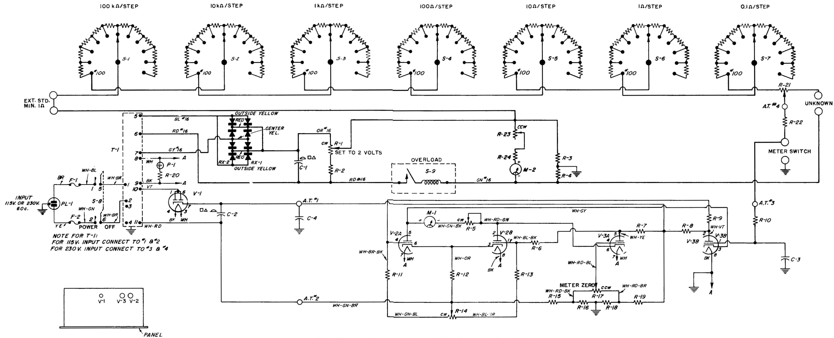
Figure 3-1. Schematic diagram for the Type 1652-A Resistance Limit Bridge.
