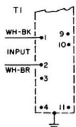
Figure 2-1. Input Voltage Connections. For 115-volt operation, connect to 1 and 2. For 230-volt operation, connect to 3 and 4.
