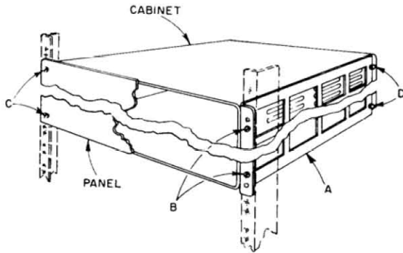
Figure 2-2. Installation of relay-rack model, Type 1652-AR.
