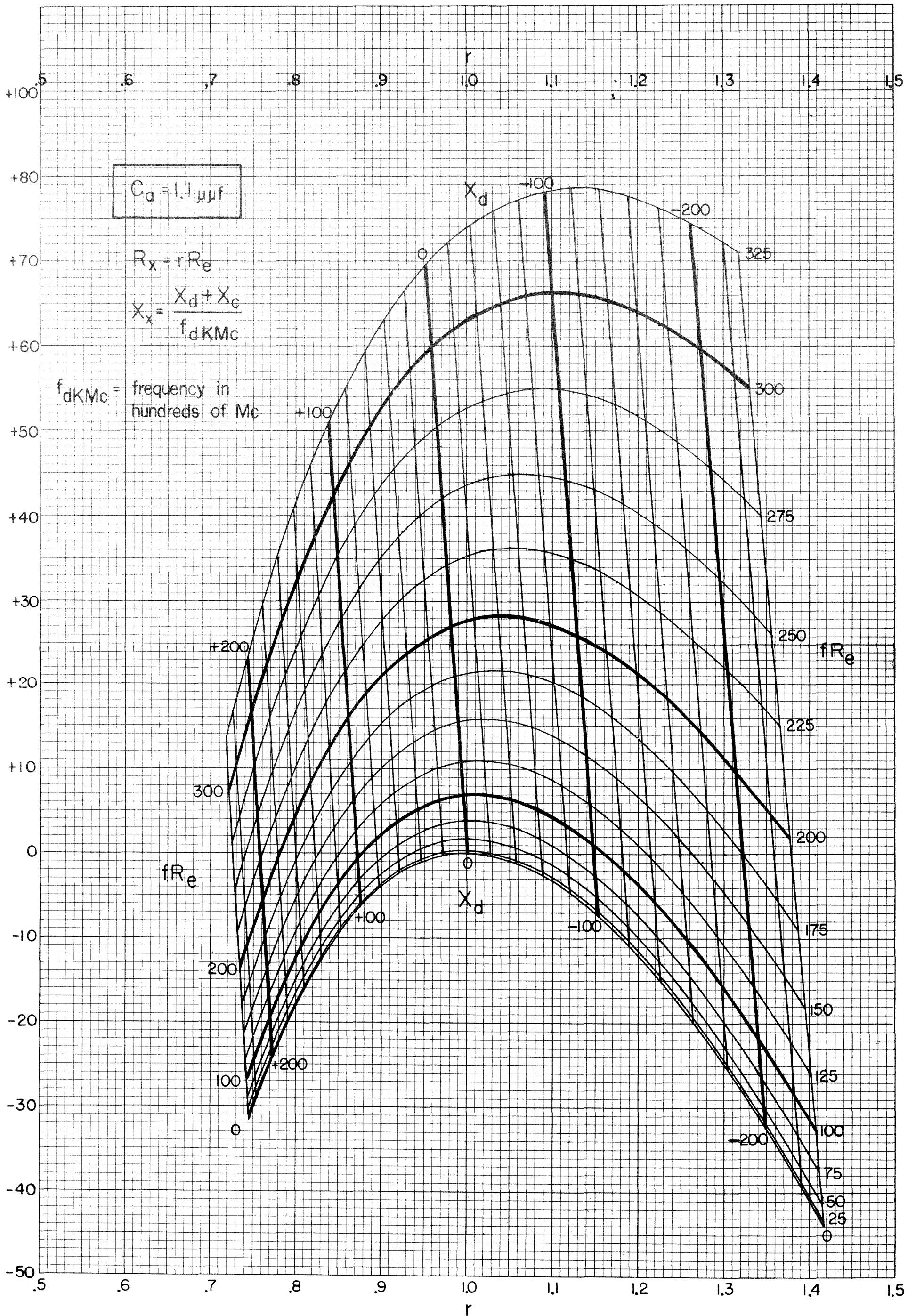
Figure 10. Correction Chart for Terminal Capacitance.
