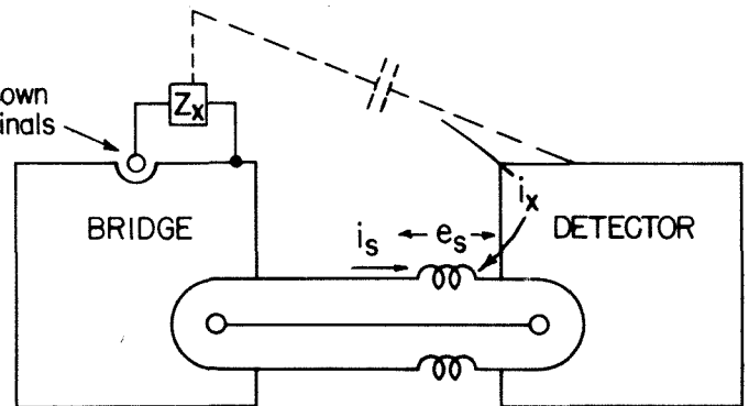
Figure 7. Sketch Showing Effect of Leakage in Coaxial Connections between Detector and Bridge.
