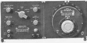
(Right) Rack-mount version (Type 1209-C4R) of the combination shown above.
