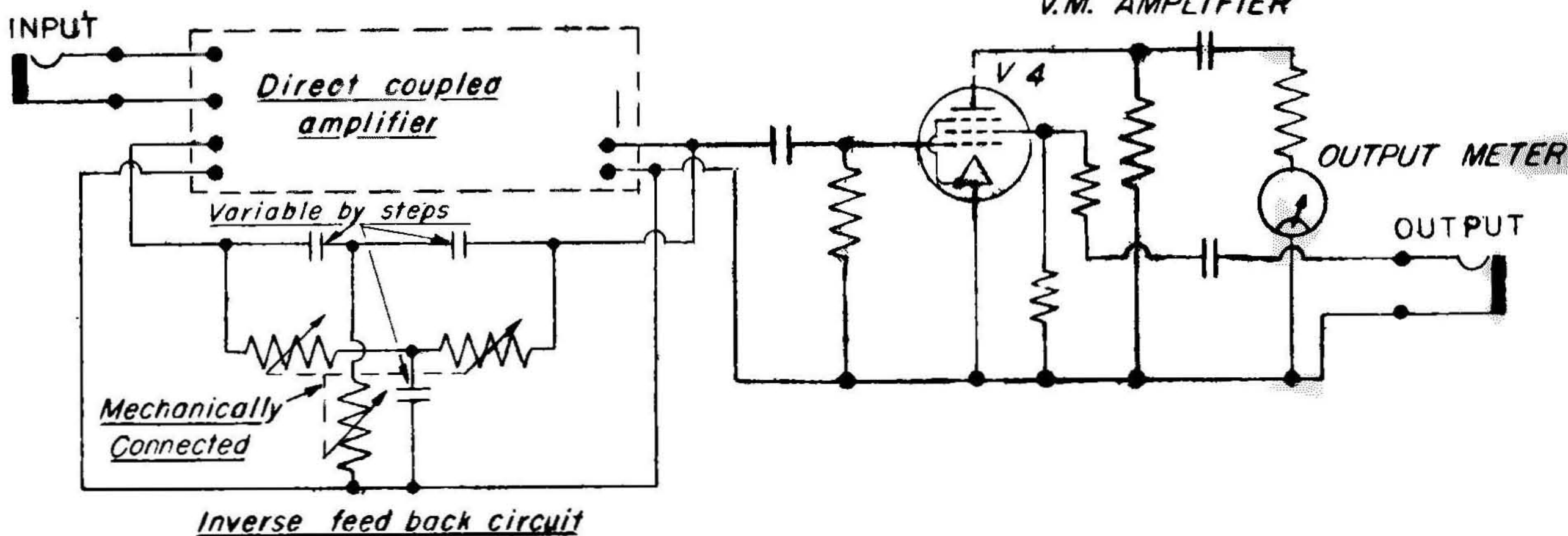
Figure 3. Schematic Diagram of Type 760-B Sound Analyzer.
