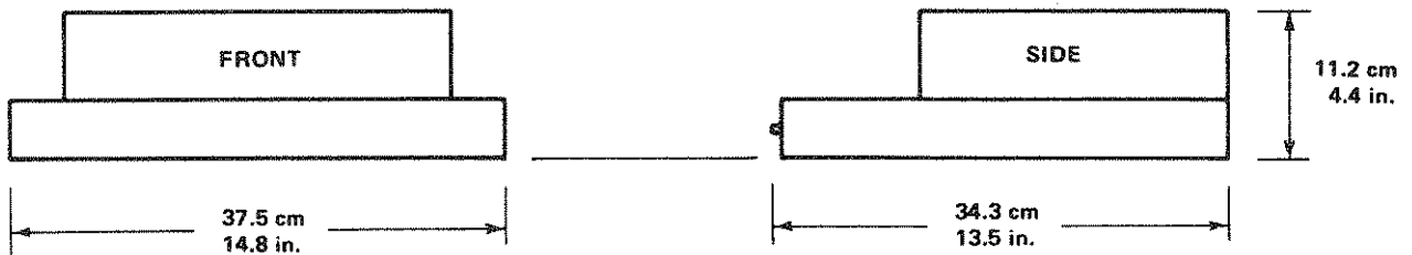
Figure 2-1. Overall dimensions.
