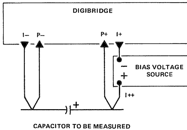
Figure 2-2. Connection of a bias voltage source to enable measurement of capacitors with bias applied. Because the measurement current (up to 30 mA rms) must pass through the bias source, it must be capable of being both source and sink for peaks of about 45 mA. Observe the voltage limits and procedural warnings in the text. Refer to the text also for discharge circuitry.
