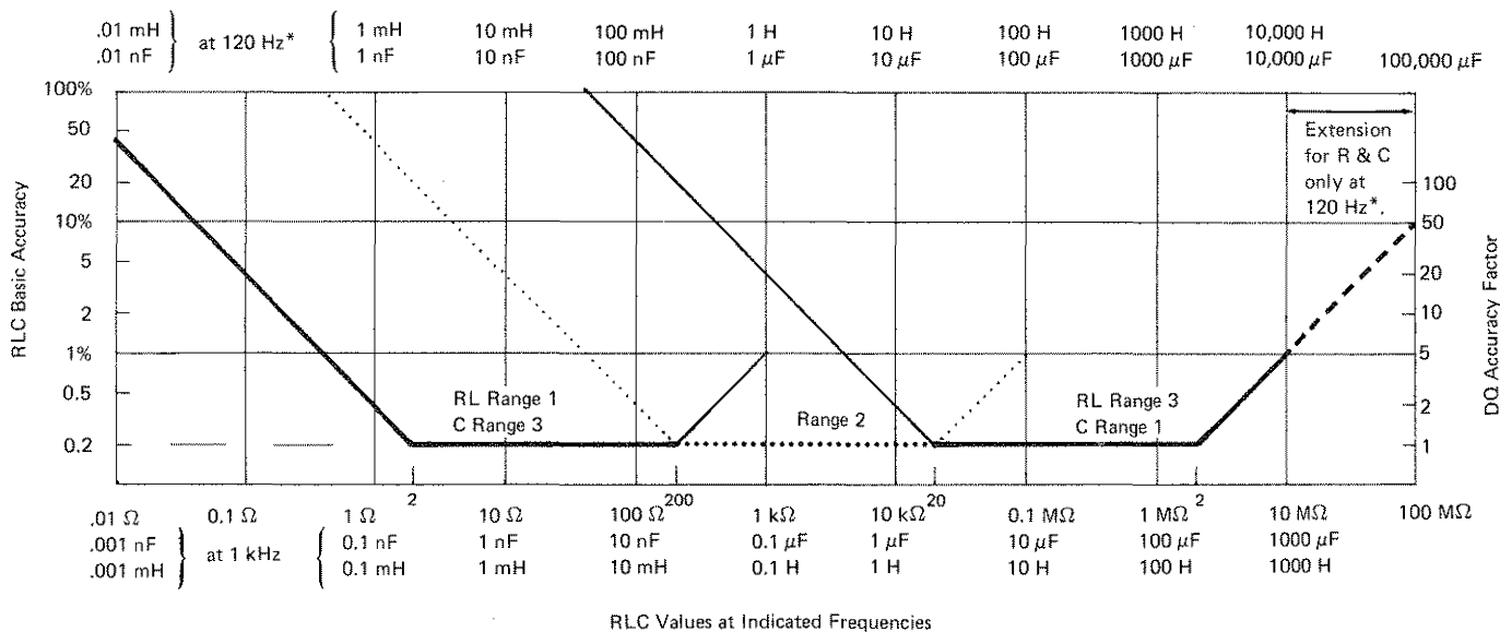
Figure 3-2. R L C basic accuracy as a percent of reading. Heavy lines (solid and dotted) represent best choice of range. Range 2 is dotted. Notice that L and C scales above graph are for 120 Hz (*equally valid for 100 Hz) and the 2 below graph are for 1 kHz. The DQ accuracy factor (right-hand scale) is the multiplier that, applied to the DQ Basic Accuracy, yields complete DQ accuracy, for range extensions as well as the basic ranges (where RLC accuracy is 0.2%).
