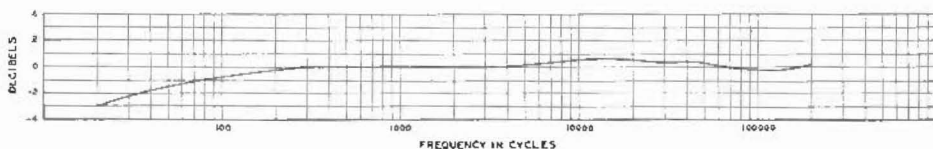
Frequency characteristic TYPE 741-G Line-to-Grid Transformer. Voltage step-up ratio 1:3.4
