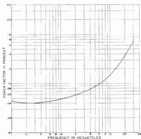
Change in power factor with frequency for a 500 \mu\mu\text{f} condenser
