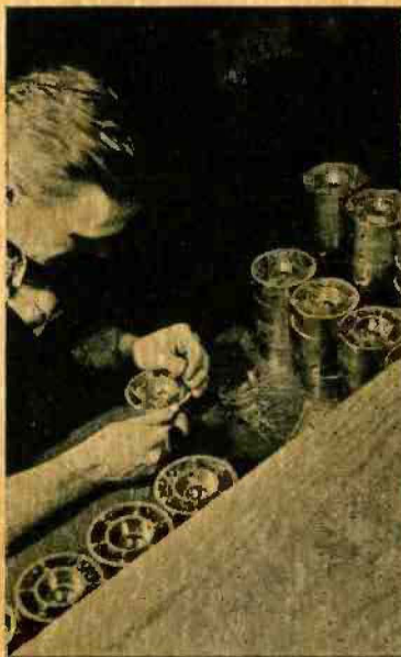
6 - ASSEMBLING ATTENUATOR HOUSINGS
