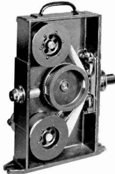
Interior View of the High-Speed Camera
