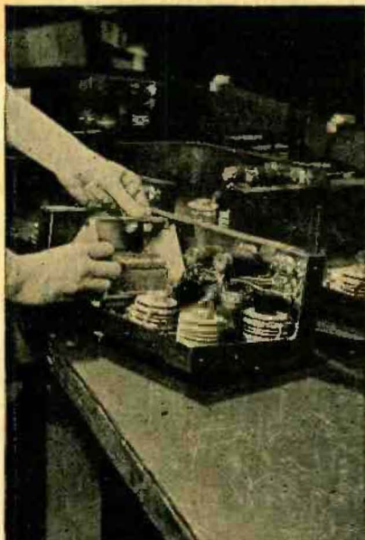
22 - FINAL OSCILLATOR ASSEMBLY
