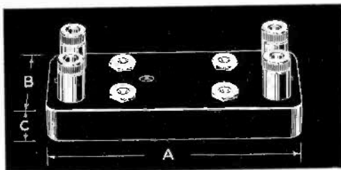
Type 274-RJ Four-Gang Jack Base
