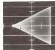
(Left) Amplitude modulation characteristic at 900 megacycles. Peak r-f output is 10 millivolts; r-f input, 50 millivolts. (Right) Oscilloscope showing modulation pulse and r-f output pulse. Pulse duration is 0.25 \mu sec with 0.05 \mu sec rise time. Carrier frequency is 60 megacycles. Scale is 0.1 \mu sec per horizontal division.
