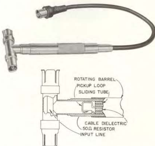
Cross section of the coupling system used in the TYPE 874-GA Adjustable Attenuator.
