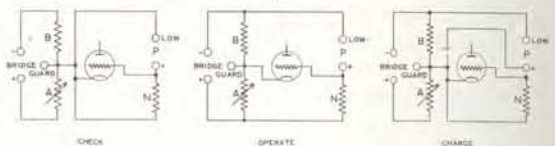
Schematic diagrams of the megohm bridge.
