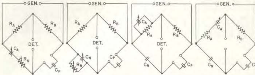
FIGURE 3. Four basic methods of obtaining resistance balance.
