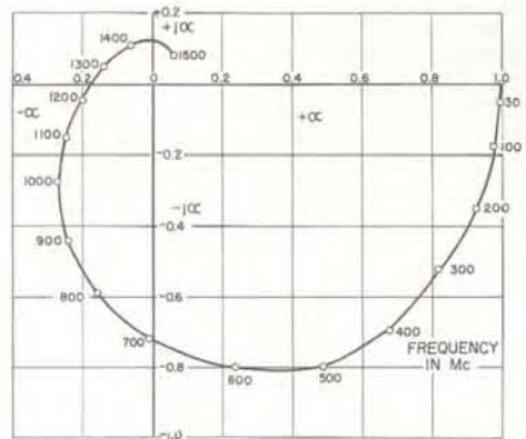
Plot of alpha versus frequency for a 1957 experimental, high-frequency transistor supplied by Bell Telephone Laboratories (Grounded base connection).
