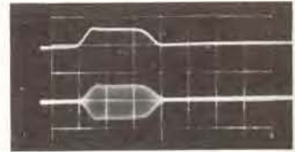
(Left) Amplitude modulation characteristic at 900 megacycles. Peak r-f output is 10 millivolts; r-f input, 50 millivolts. (Right) Oscilloscope showing modulation pulse and r-f output pulse. Pulse duration is 0.25 \mu sec with 0.05 \mu sec rise time. Carrier frequency is 60 megacycles. Scale is 0.1 \mu sec per horizontal division.
