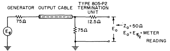
Figure 5b. Wiring Diagram of Type 805-P2, 50-ohm Termination Unit.
