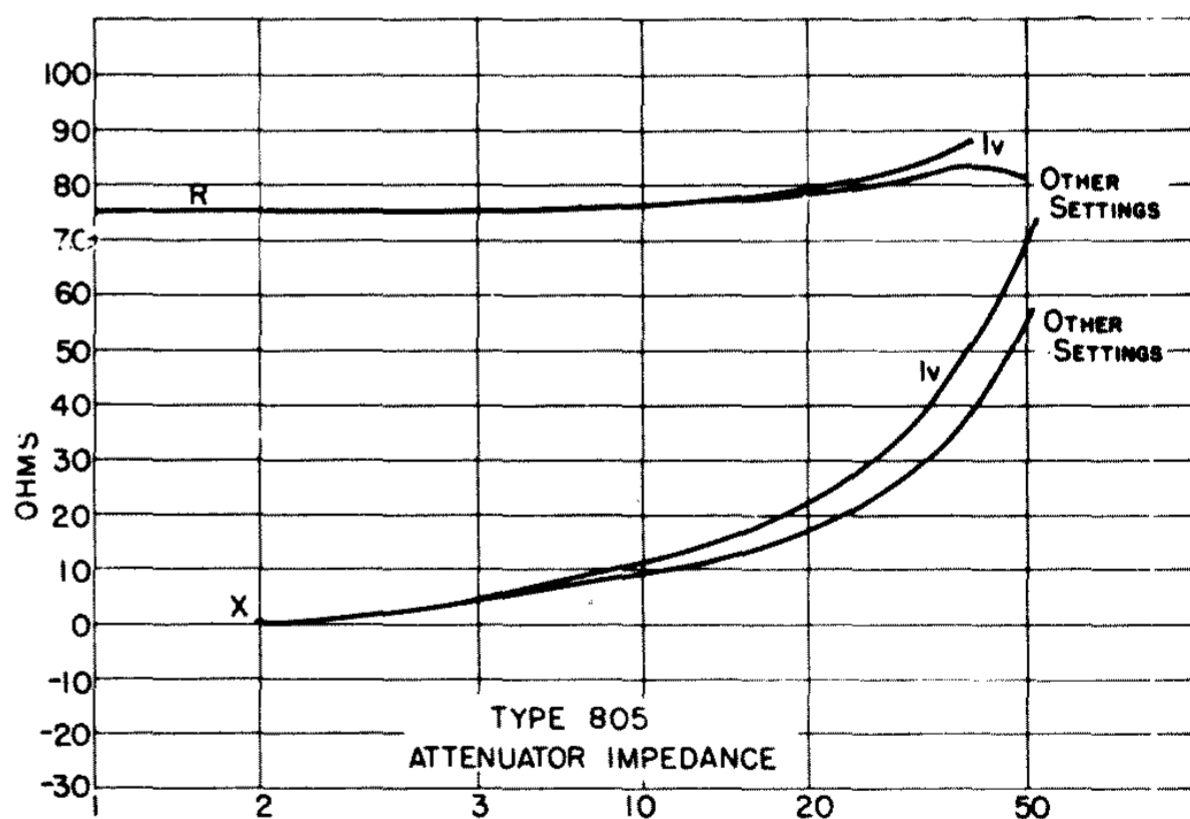
Figure 11. Attenuator impedance as a function of frequency.
