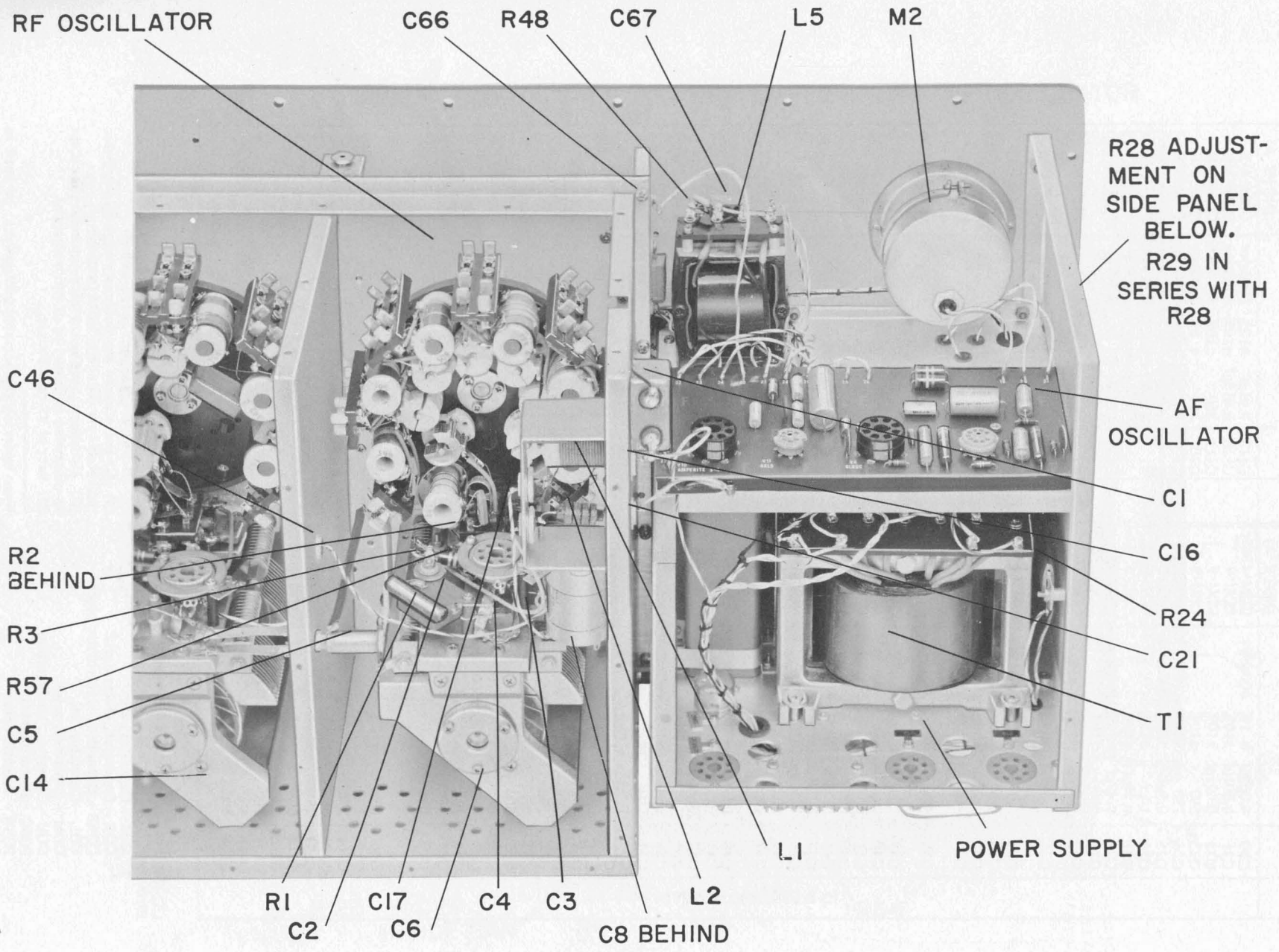
FIGURE 13. VIEW OF POWER SUPPLY AND CARRIER OSCILLATOR WITH PARTS IDENTIFICATION.
