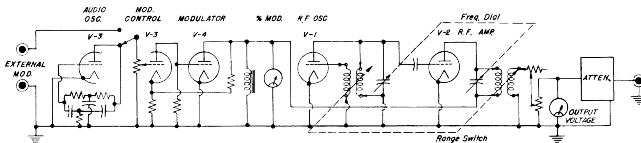
Figure 1. Elementary Schematic Diagram.
