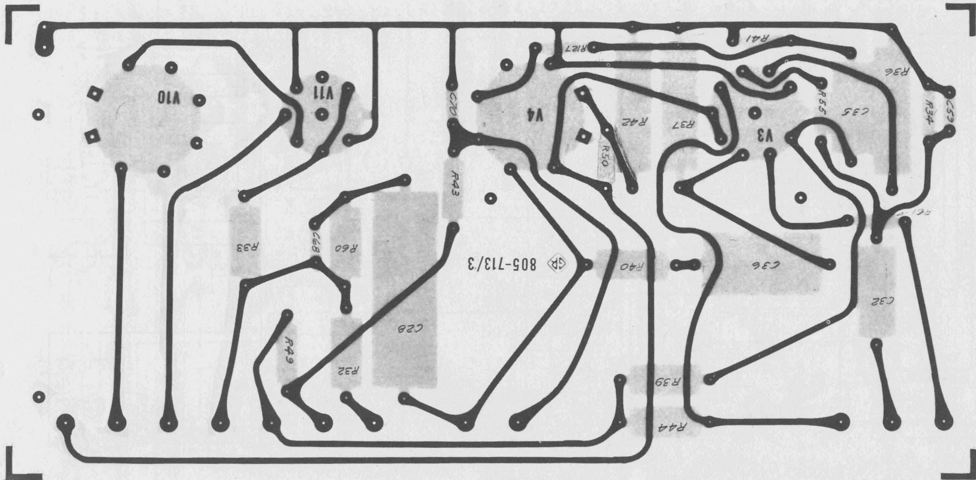
COMPONENT LAYOUT ON ETCHED BOARD
