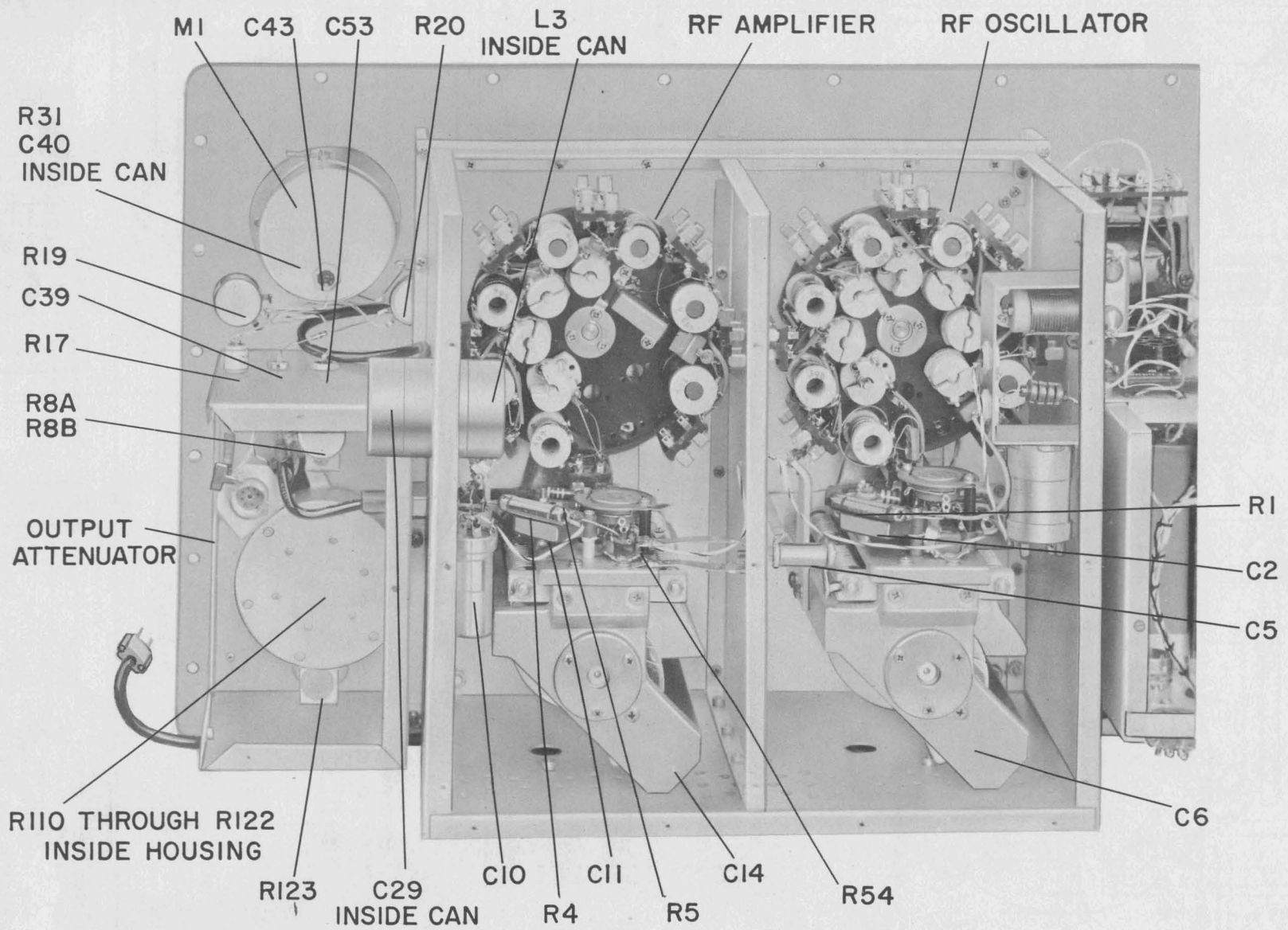
FIGURE 14. VIEW OF R-F AMPLIFIER AND OUTPUT SYSTEM WITH PARTS IDENTIFICATION
