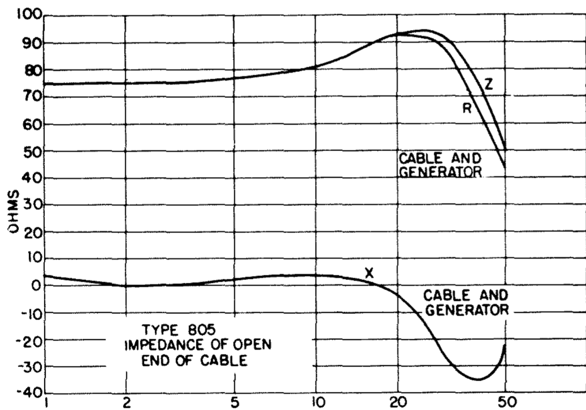
Figure 10. Output impedance at open end of cable.
