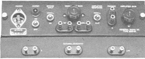
FIGURE 2. Panel view of the TYPE 650-P1 Oscillator-Amplifier, showing top of bridge panel. Connections are easily made from either the d-c or 1000-cycle terminals to the EXTERNAL GENERATOR terminals of the bridge.
