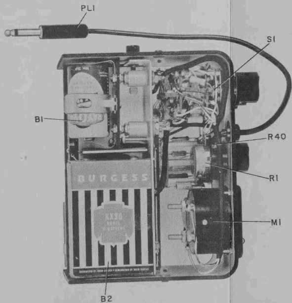
Figures 7 and 8. Interior Views. (Insets show rear views of switches.)
