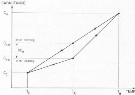
Figure 2. Capacitance vs temperature diagram showing hysteresis.
