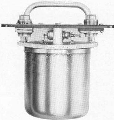
Figure 4. View of capacitor with cabinet removed, showing the sealed container and the three-terminal trimmer.
