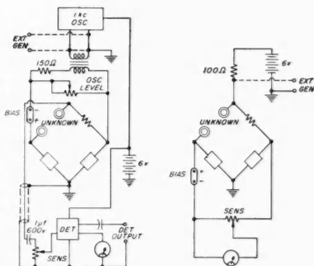
Figure 3. Block schematic of the bridge generator and detector. External-generator connections are shown by dashed lines.
