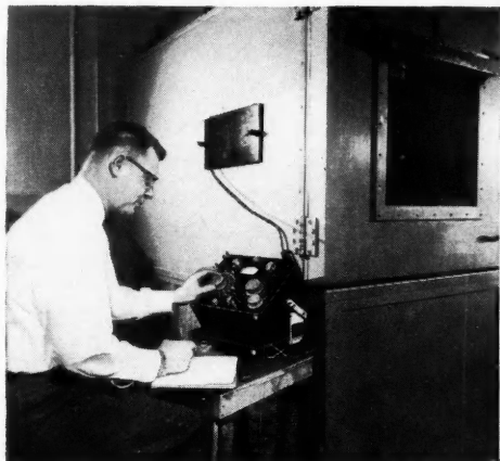
Figure 11. Bridge in use for 3-terminal measurements of sample in conditioning chamber.
