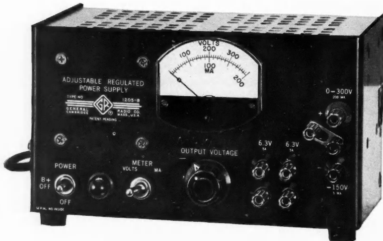
Figure 1. Panel view of the Adjustable Regulated Power Supply.
