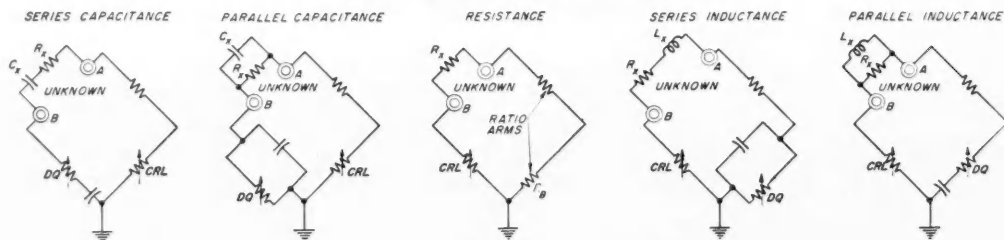
Figure 2. The five circuits used in the bridge.
