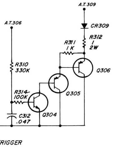
Figure 6-9. Schematic diagram of the high-voltage supply, guard, trigger and generator circuits.
