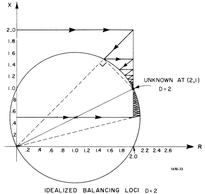
Figure 5-10. Loci of "sliding null" balances.
