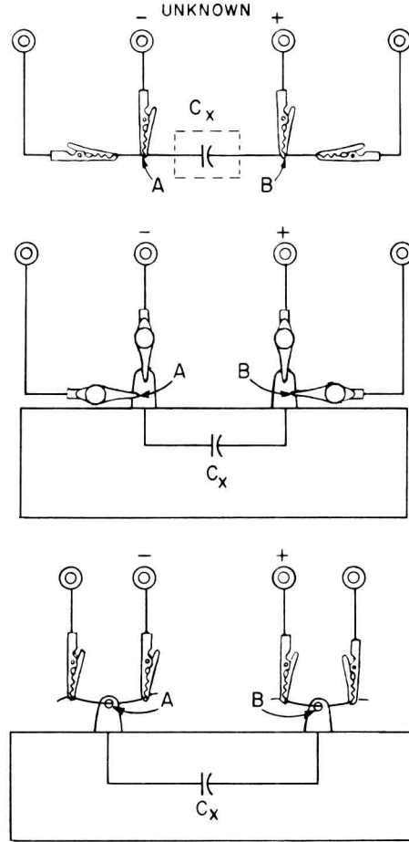
Figure 3-4. Different types of 4-terminal connections. The unknown is measured from A to B.
