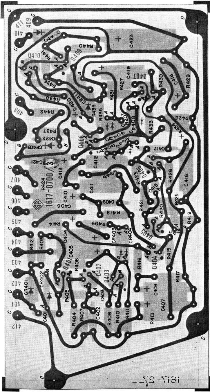
Figure 6-10. The detector etched board, (P/N 1617-2770) for 50-Hz units or P/N 1617-2700 (for 60 Hz units).
