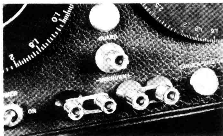
Figure 3-1. UNKNOWN and GUARD terminals on the bridge.
