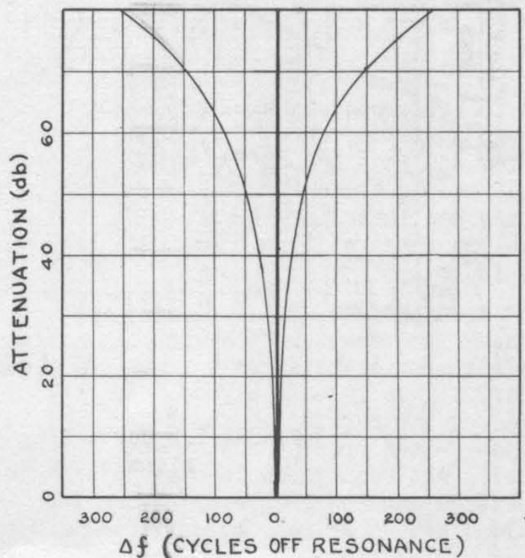
FIGURE 6. Over-all response characteristic of the quartz-crystal filter.
