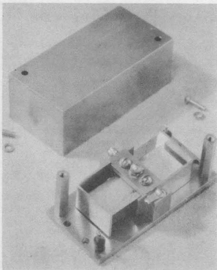
FIGURE 4. One of the 50-kc quartz bars
