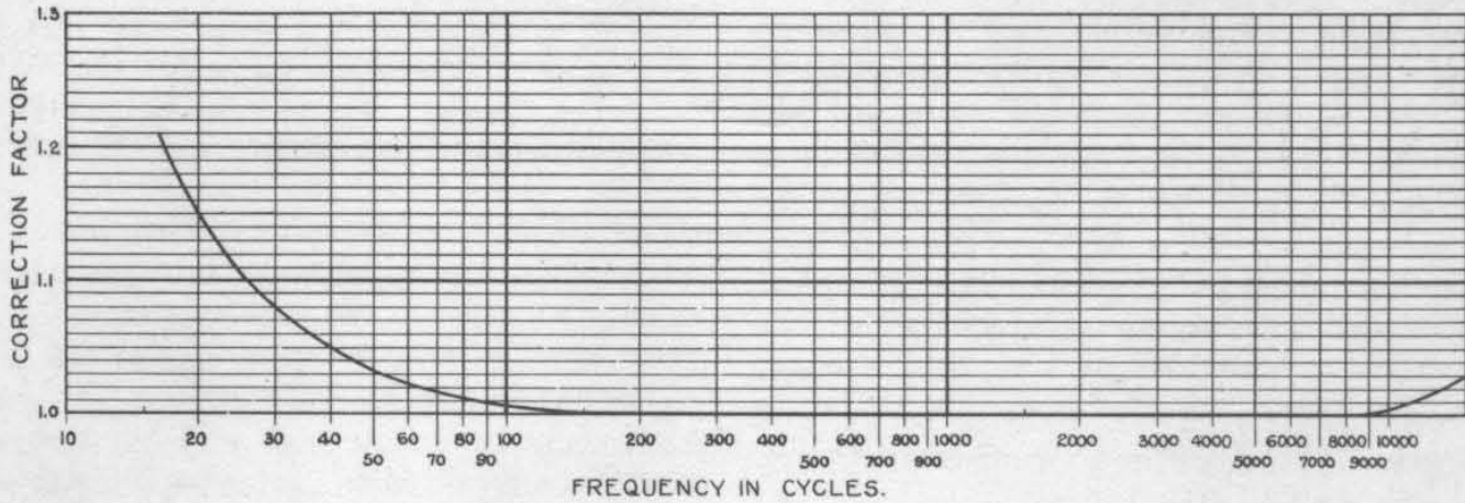
FIGURE 5. Frequency characteristic. See 4.5
