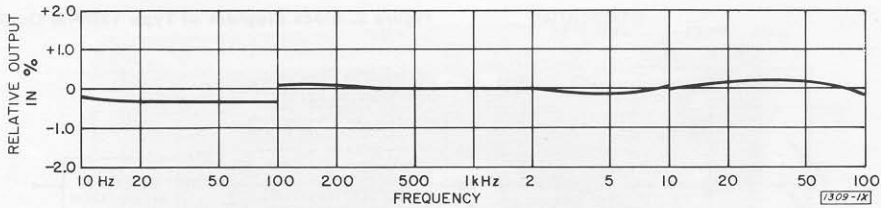
Figure 4. Typical oscillator output voltage versus frequency.
