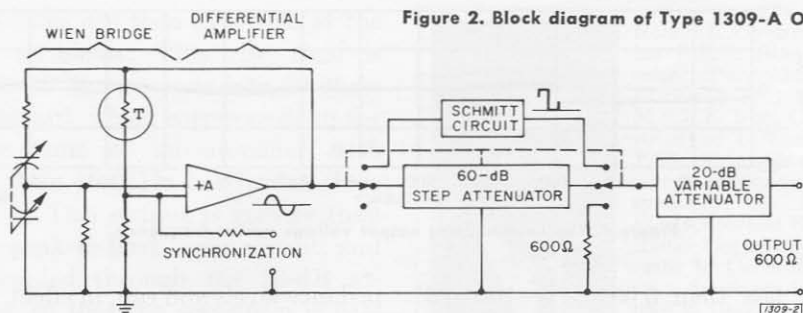
Figure 2. Block diagram of Type 1309-A Oscillator.
