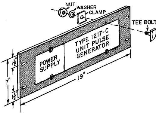
Figure 2-3. Rack-mounting the Type 1217-C/ power supply combination by means of a Type 480-P4U3 Relay-Rack Adapter Set.
