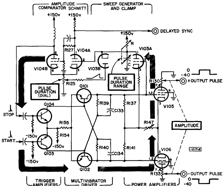
Figure 3-5. Simplified schematic diagram of the output pulse circuit.
