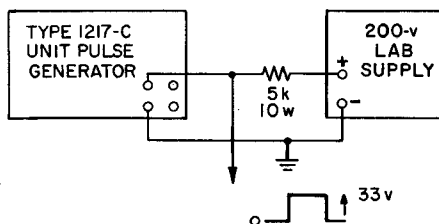
Figure 2-10. Connection for translating pulse dc component by means of external power supply.
