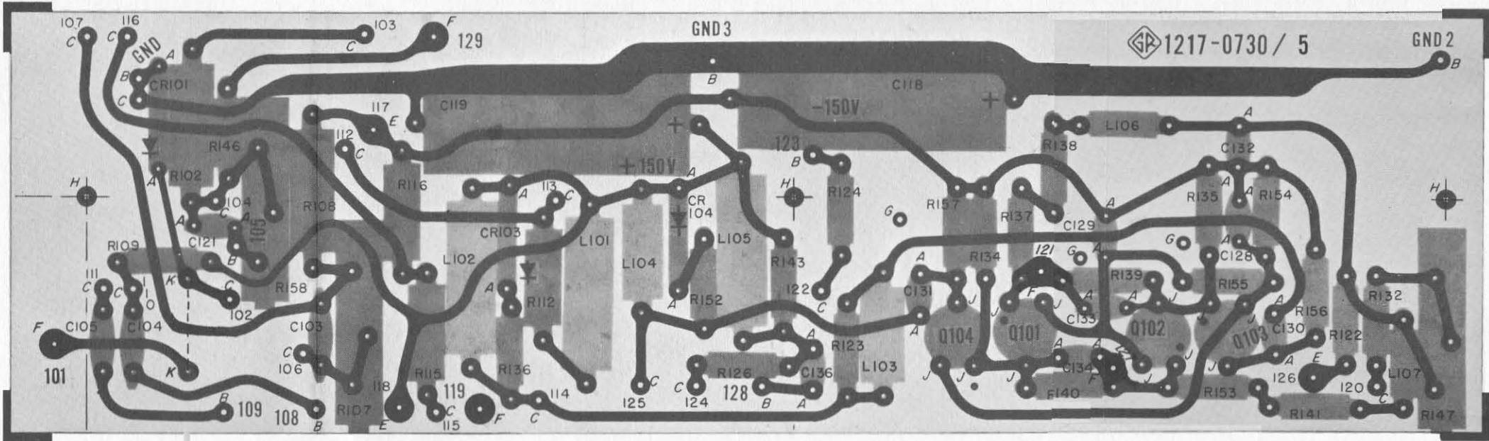
Figure 4-6. PCB layout. File Courtesy of GRWiki.org
