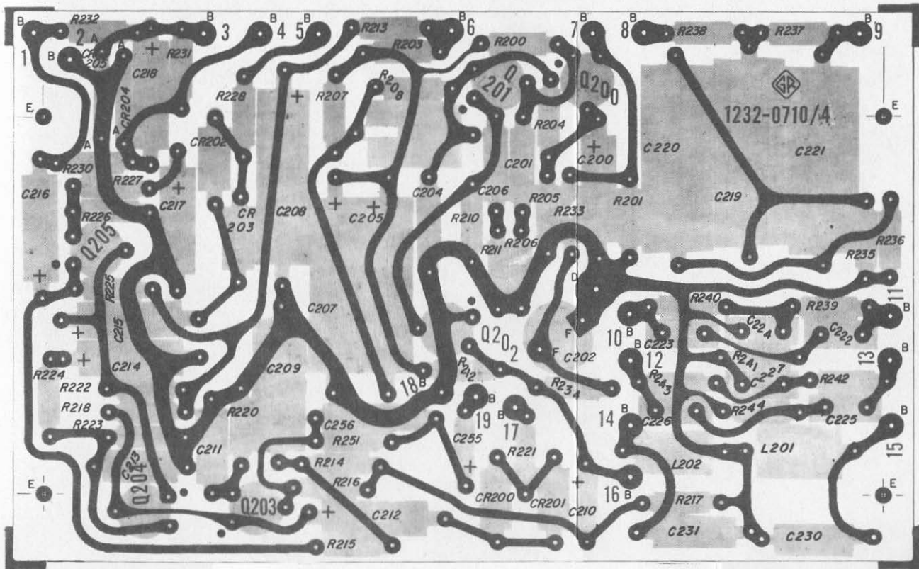
Figure 13. Etched Board Layout of the Type 1232-A Tuned Amplifier and Null Detector, P/N's 1232-2700 and 1232-2710.
