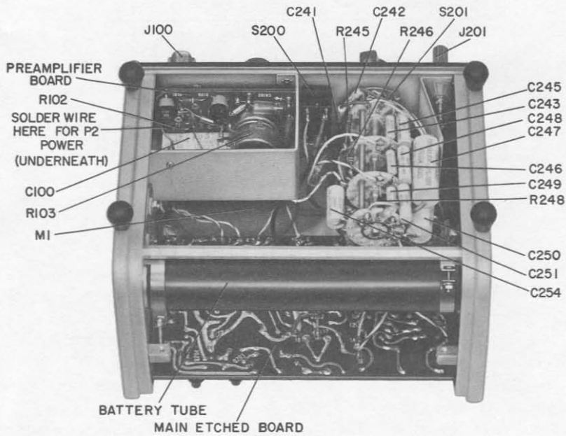
Figure 8. Bottom interior view of the Type 1232-A.
