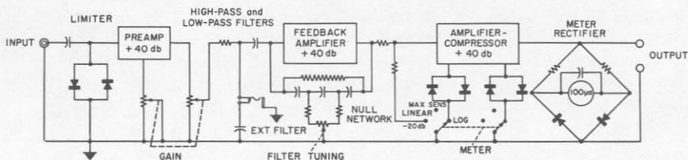
Figure 2. Functional diagram of the null detector.
