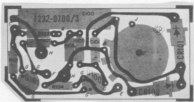
Figure 13. Etched Board Layout of the Type 1232-A Tuned Amplifier and Null Detector, P/N's 1232-2700 and 1232-2710.
